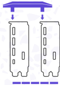
3-Slot spacing 100-2W-0029-LR
